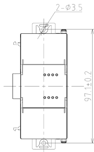
Figure 157 Mounting Dimensions
