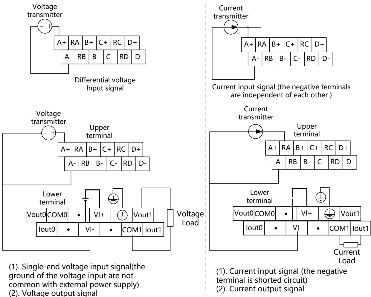
Figure 105 Terminal Definition and Field Wiring
