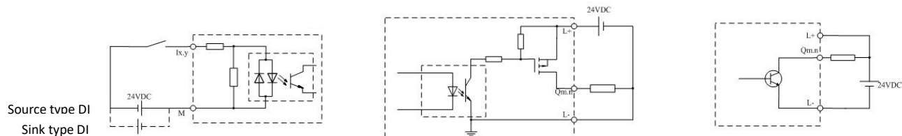
Figure 46 Input Channel
