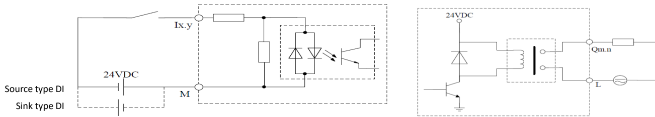
Figure 58 Electrical Schematic Diagram of Input Electrical Schematic Diagram of Output
