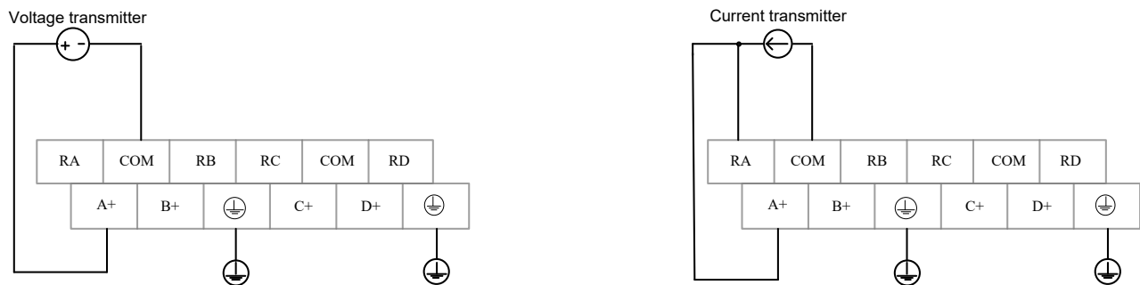
Figure 94 Upper Terminals Definition and Wiring (voltage type) Upper Terminals Definition and Wiring (current type)
