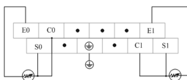
Figure 98 Upper Terminal Definition and Wiring
