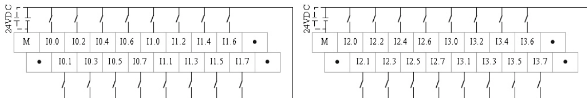
Figure 81 Upper Terminal Definition and Wiring
