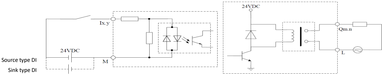
Figure 41 Electrical Schematic Diagram of Input Electrical Schematic Diagram of Output
