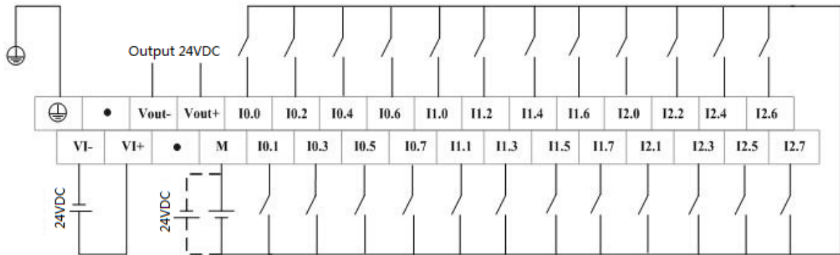
Figure 42 Upper Terminal Definition and Wiring
