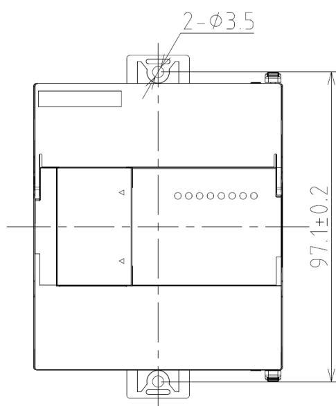
Figure 159 Mounting Dimensions
