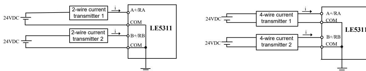
Figure 96 2-wire Type and 4-wire Type Wiring
