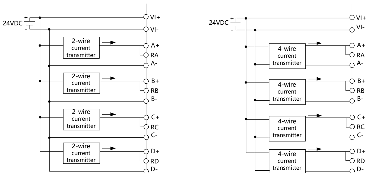
Figure 106 2-wire Type and 4-wire Type Wiring
