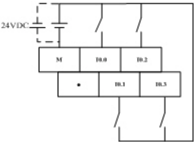
Figure 65 Terminal Wiring
