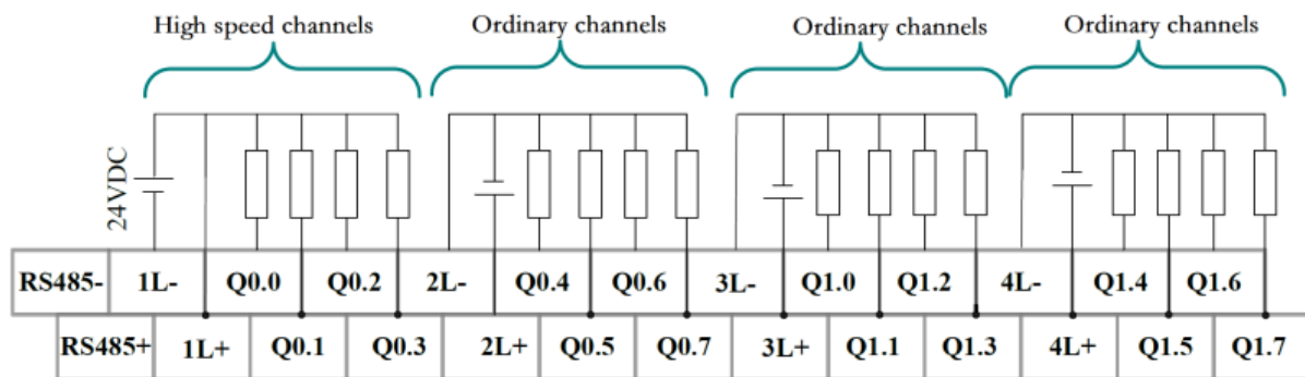
Figure 43 Lower Terminal Definition and Wiring
