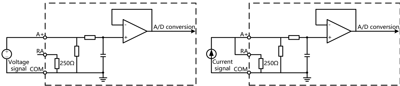
Figure 16 Single-end Analog Input Channels
