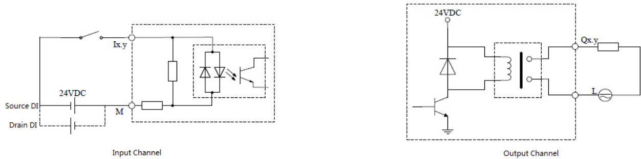
Figure 90 Electrical Schematic Diagram
