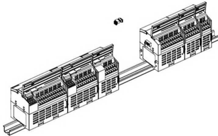
Figure 88 Expansion Connection
