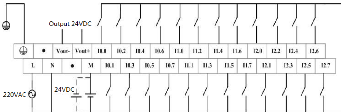
Figure 56 LE5119 Upper Terminals Definition and Wring Diagram
