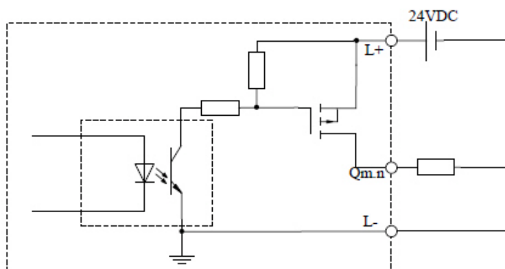
Figure 70 Electrical Schematic Diagram
