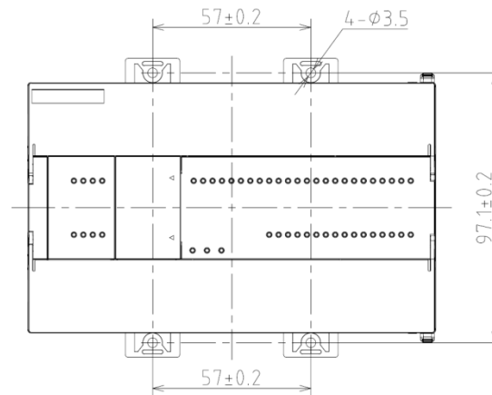
Figure 151 Mounting Dimensions
