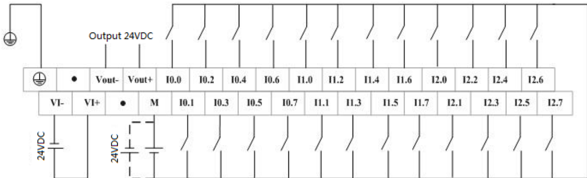
Figure 50 Upper Terminal Definition and Wiring
