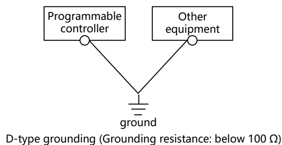
Figure 147 Grounding Diagram
