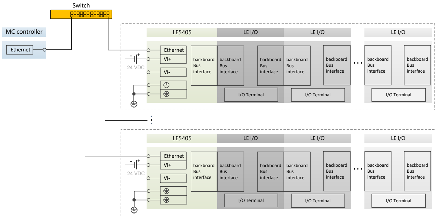
Figure 125 Wiring Schematic
