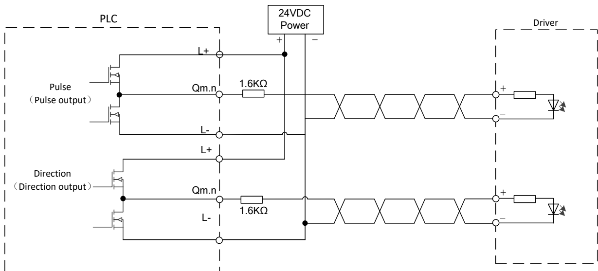
Figure 52 CW/CCW Mode Wiring Diagram
