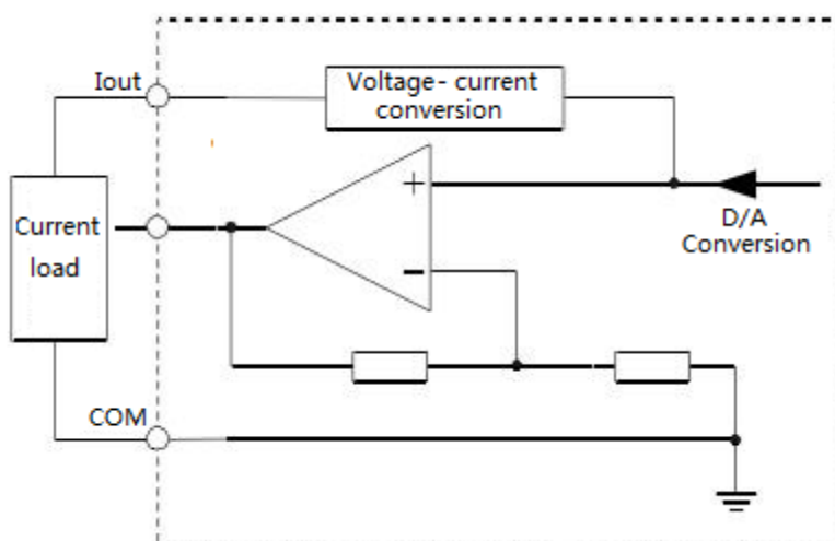
Figure 39 Output Channel (AO)
