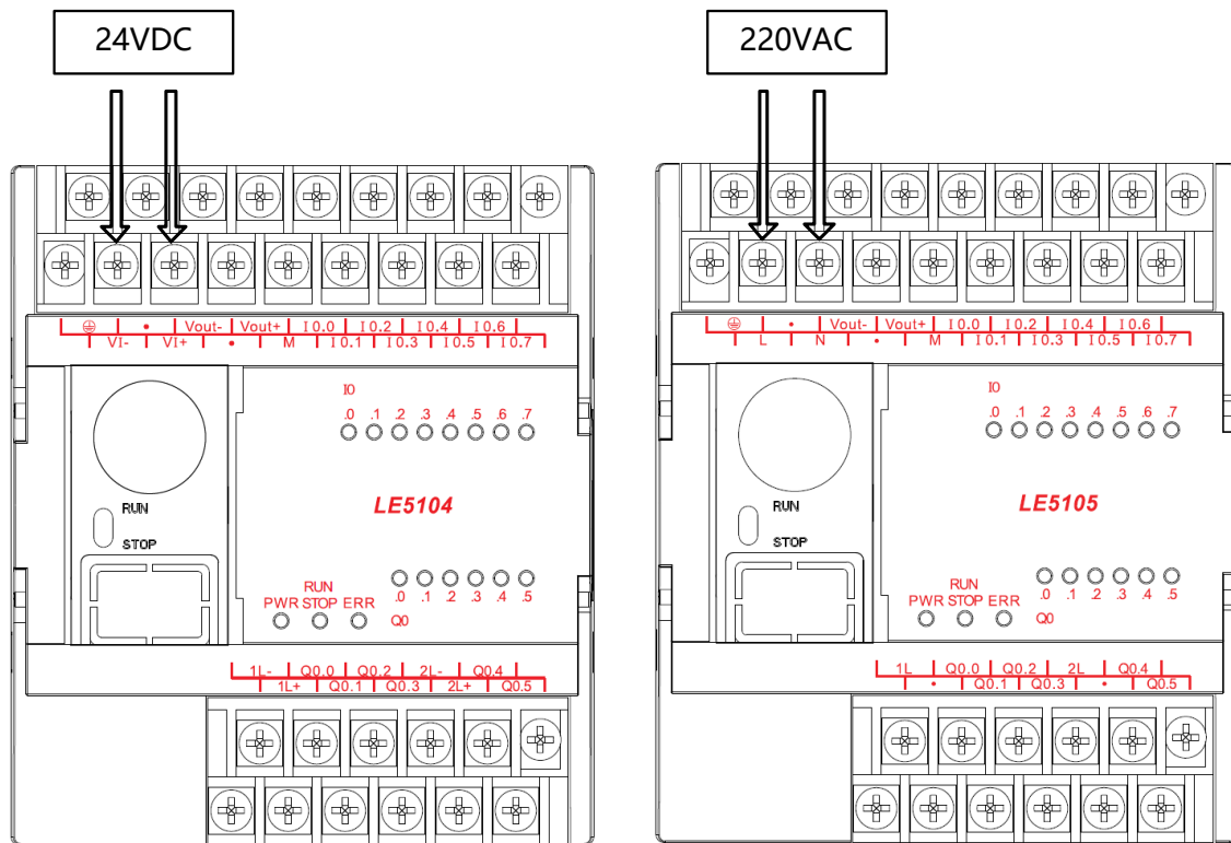
Figure 22 Power Supply Wiring Diagram
