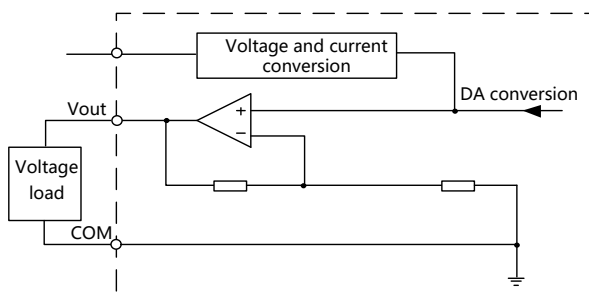
Figure 78 Voltage-Type Load Output
