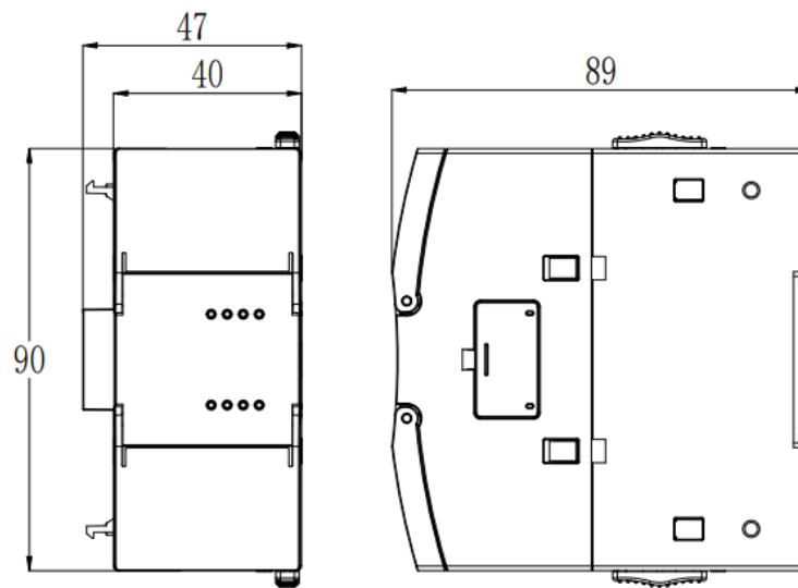
Figure 156 Outline Dimensions
