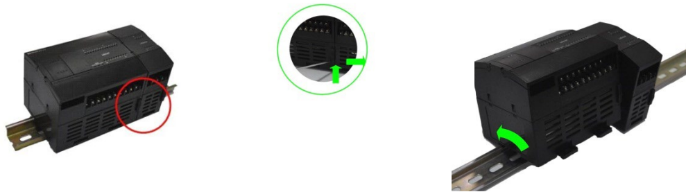
Figure 136 Diagram of Opening the Bottom Side Locker
