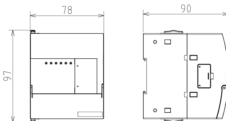
Figure 158 Outline Dimensions
