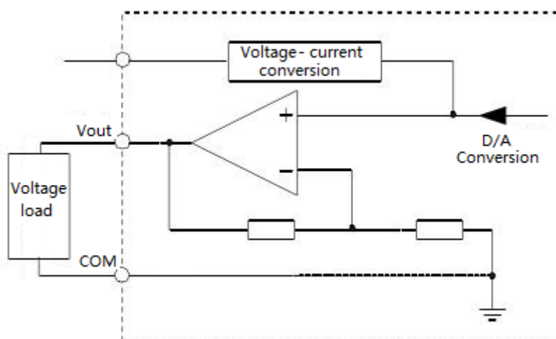
Figure 38 Output Channel (AO)
