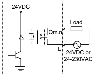
Figure 36 Output Channel (DO)
