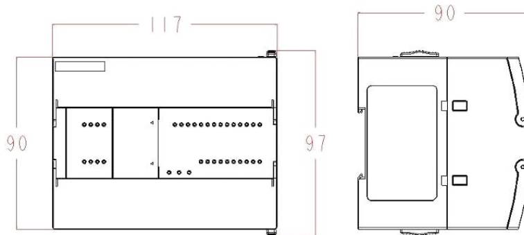
Figure 148 Outline Dimensions
