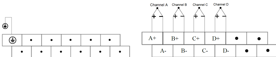
Figure 97 Upper Terminal Definition and Wiring Lower Terminal Definition and Wiring
