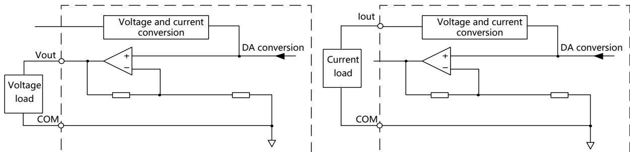
Figure 17 Electrical Schematic Diagram of Analog Output Channels
