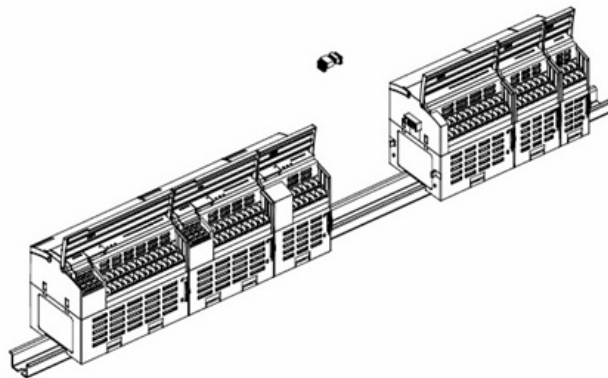
Figure 24 Module Connection
