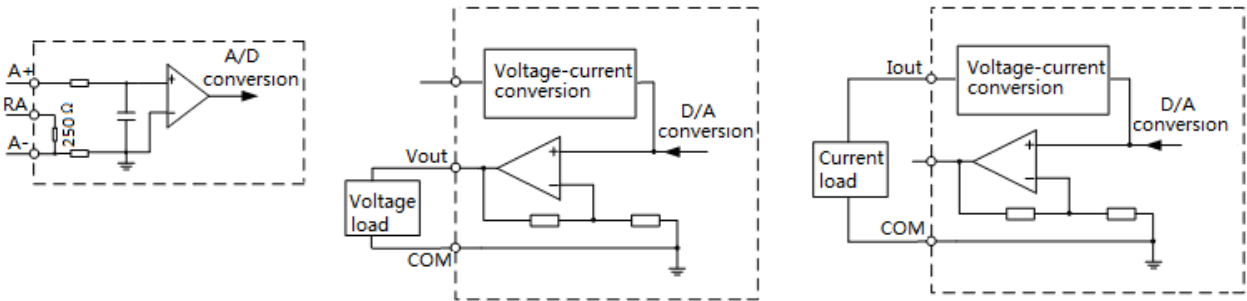
Figure 107 Input Channel Voltage Type Load Output Channel Current Type Load Output Channel
