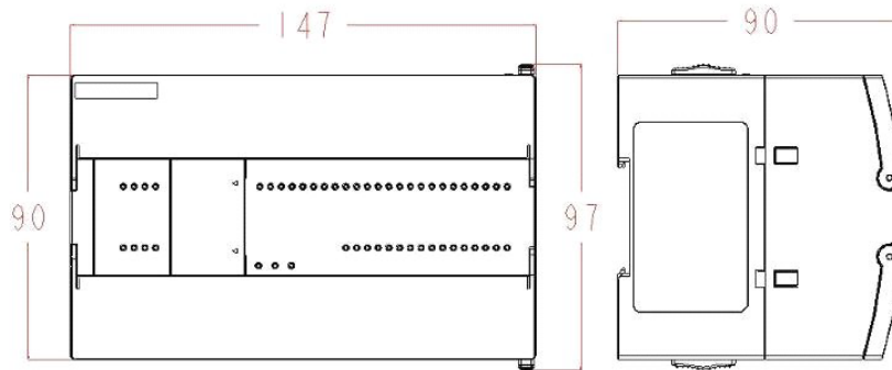
Figure 150 Outline Dimensions
