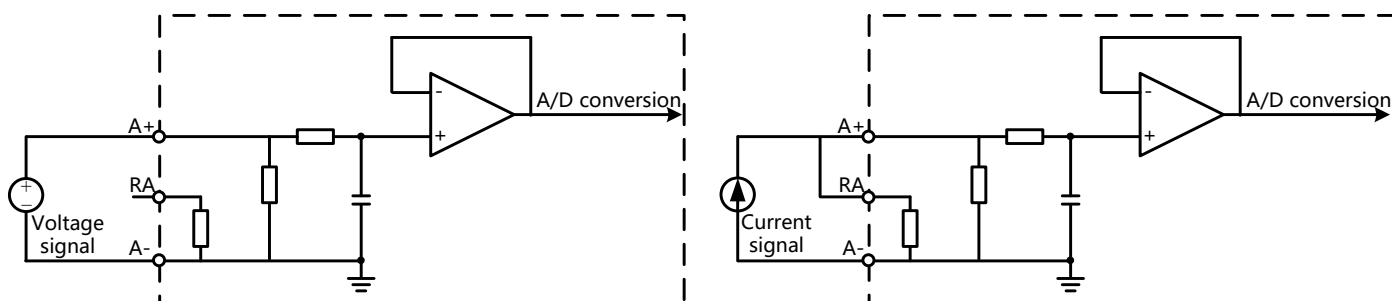
Figure 37 Input Channel (AI)
