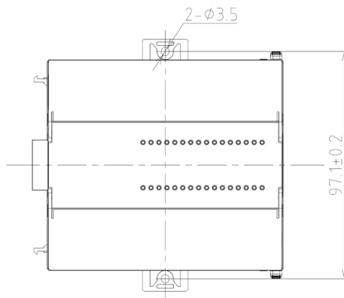
Figure 153 Mounting Dimensions
