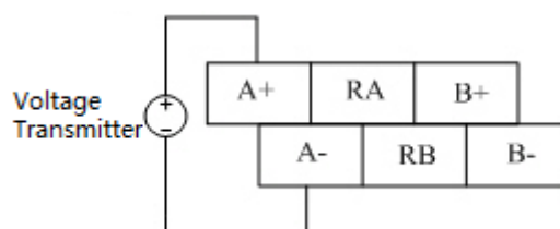
Figure 73 Terminal Definition and Wring Diagram (Voltage Type)
