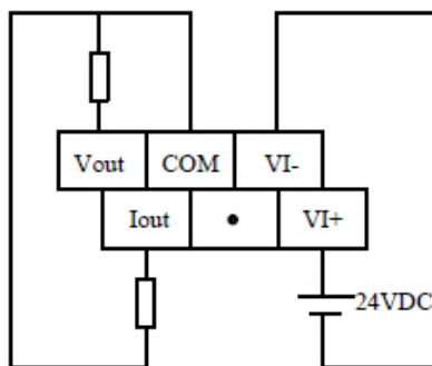
Figure 77 Terminal Wiring
