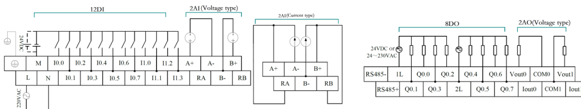
Figure 34 Upper Terminal Definition and Wring Diagram Lower Terminal Definition and Wring Diagram
