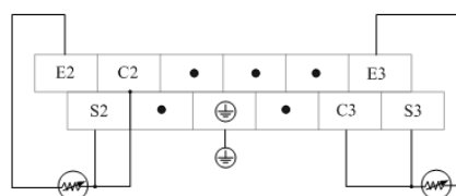
Figure 100 Lower Terminal Definition and Wiring
