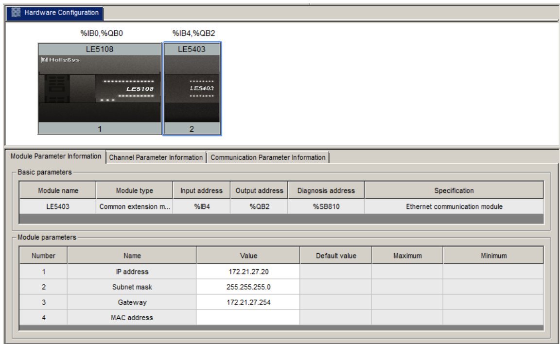
Figure 120 LE5403 Configuration
