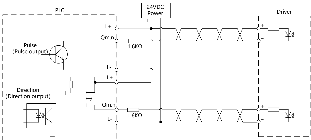
Figure 30 Pulse + Direction Mode Wiring Diagram
