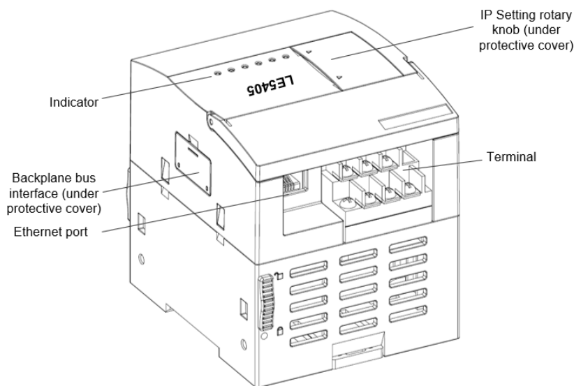
Figure 123 LE5405 Schematic
