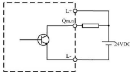
Figure 13 High-speed Transistor Digital Output Channels
