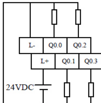
Figure 69 Terminal Wiring
