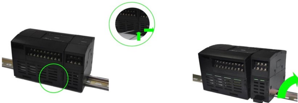
Figure 139 Removing an Expansion Module
