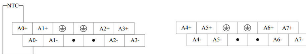
Figure 100 Terminals Schematic
