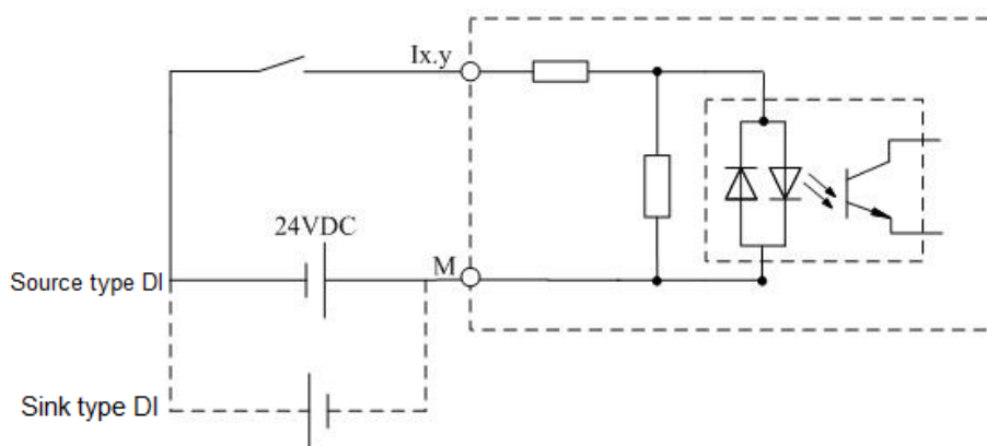
Figure 11 Digital Input Channels
