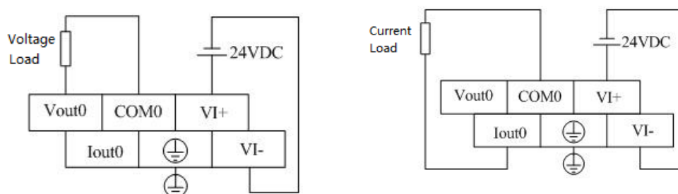
Figure 101 Upper Terminal Definition and Wiring (voltage load) Upper Terminal Definition and Wiring (current load)
