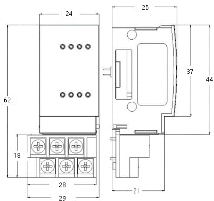
Figure 160 Outline Dimensions
