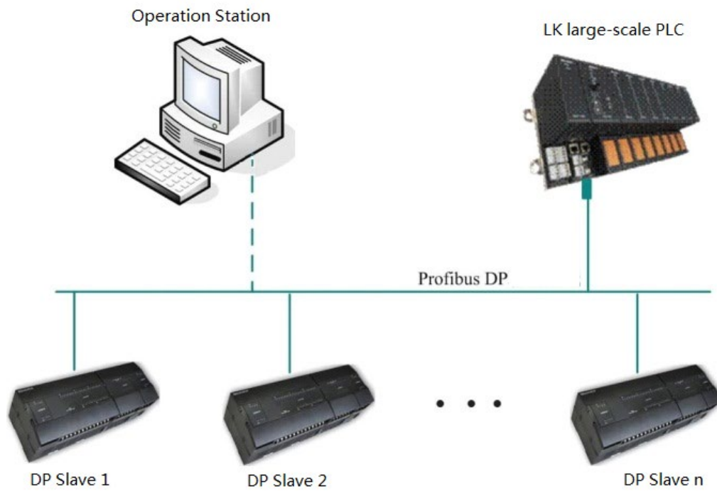
Figure 19 Profibus DP Mode
