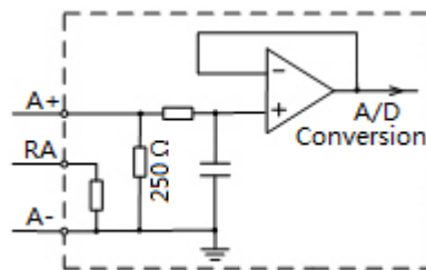
Figure 76 Electrical Schematic Diagram
