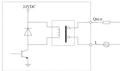
Figure 14 Relay Digital Output Channels
