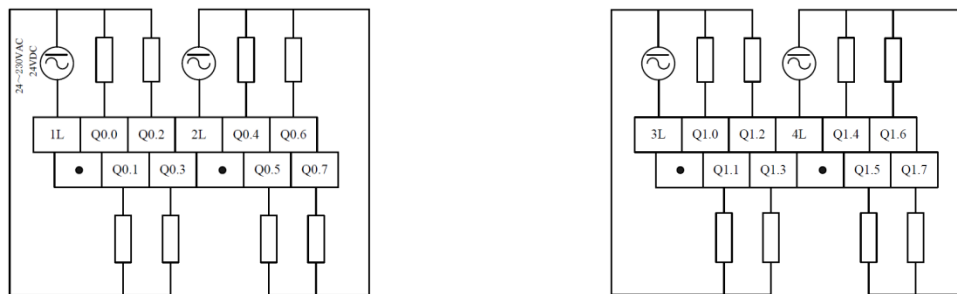
Figure 84 Upper Terminal Definition and Wiring Lower Terminal Definition and Wiring
