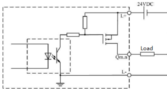
Figure 12 Ordinary Output Channels of Transistor Digital Output
