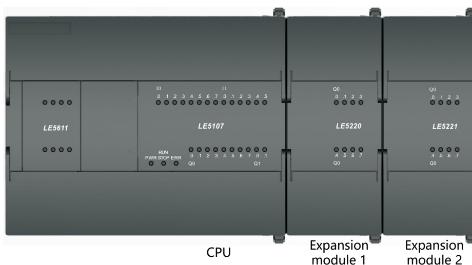
Figure 10 Expansion Module Schematic Diagram
