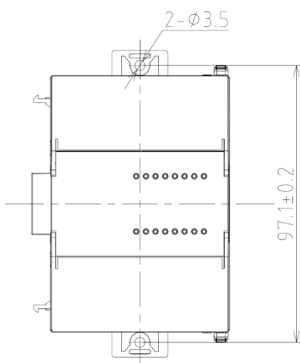
Figure 155 Mounting Dimensions
