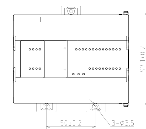
Figure 149 Mounting Dimensions
