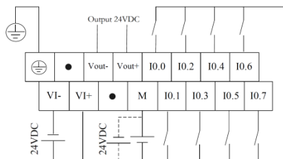
Figure 28 Upper Terminal Definition
