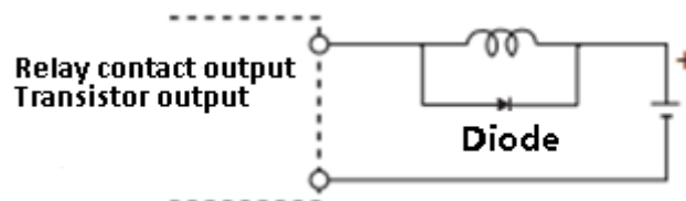
Figure 144 Typical Suppressor Circuit for Switching DC Inductive Loads
