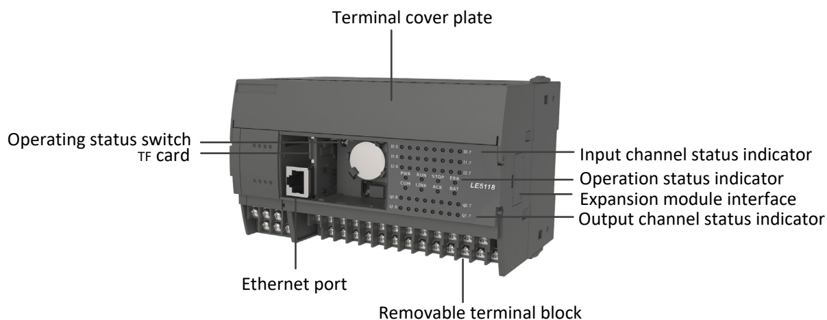
Figure 49 Module Structure
