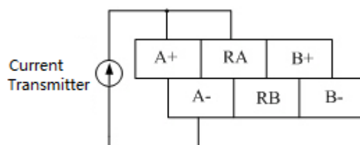
Figure 74 Terminal Definition and Wiring Diagram (Current Type)
