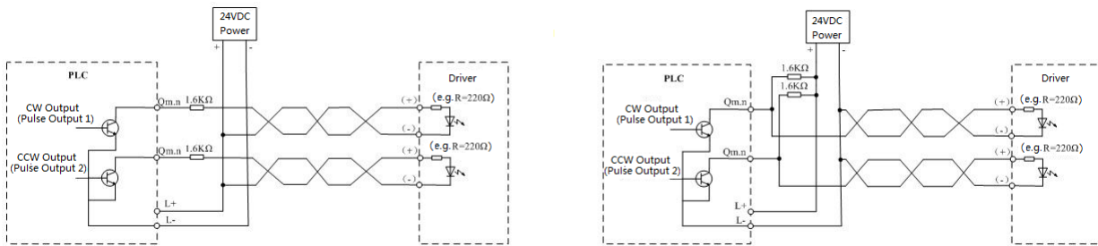
Figure 44 CW/CCW Mode Wiring Diagram
