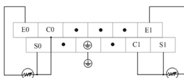
Figure 99 Upper Terminal Definition and Wiring
