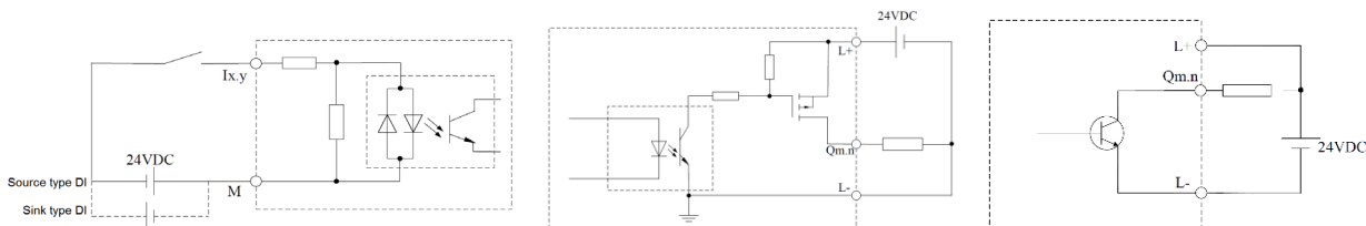
Figure 31 Input
