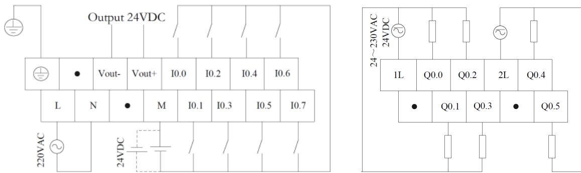
Figure 32 Upper Terminals Definition
