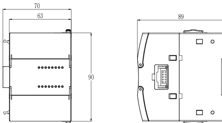
Figure 154 Outline Dimensions
