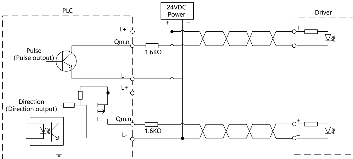
Figure 45 Pulse + Direction Mode Wiring Diagram
