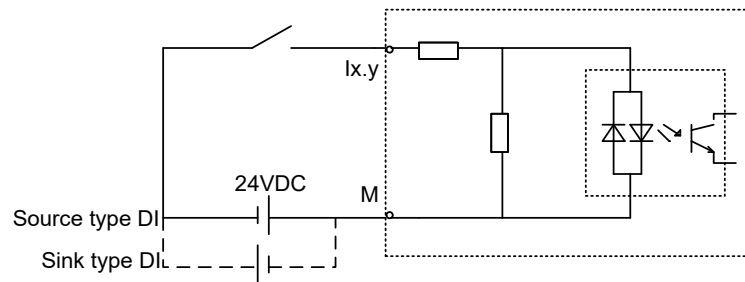
Figure 35 Input Channel (DI)
