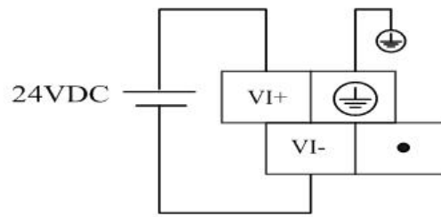
Figure 122 Terminal Wiring
