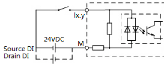
Figure 66 Electrical Schematic Diagram
