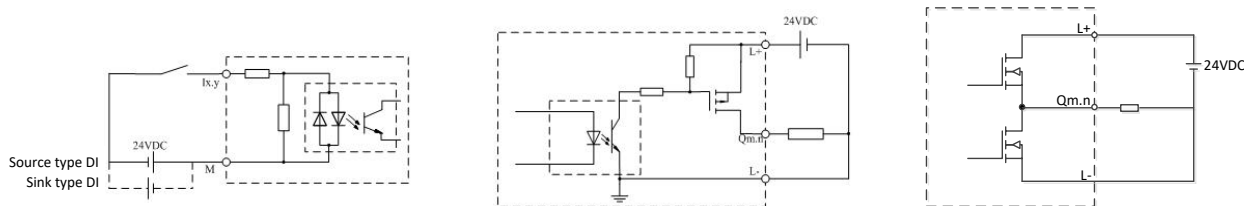
Figure 54 Input Channel
