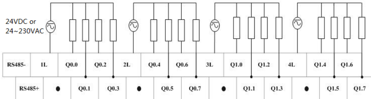
Figure 57 LE5119 Lower Terminals Definition and Wring Diagram
