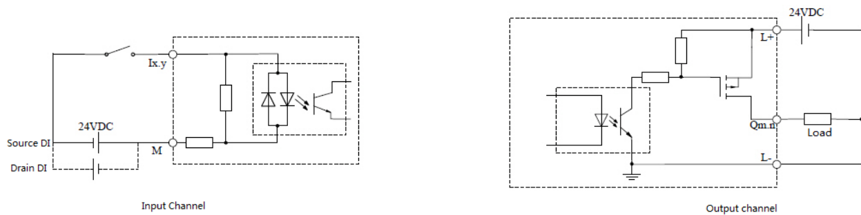
Figure 87 Electrical Schematic Diagram
