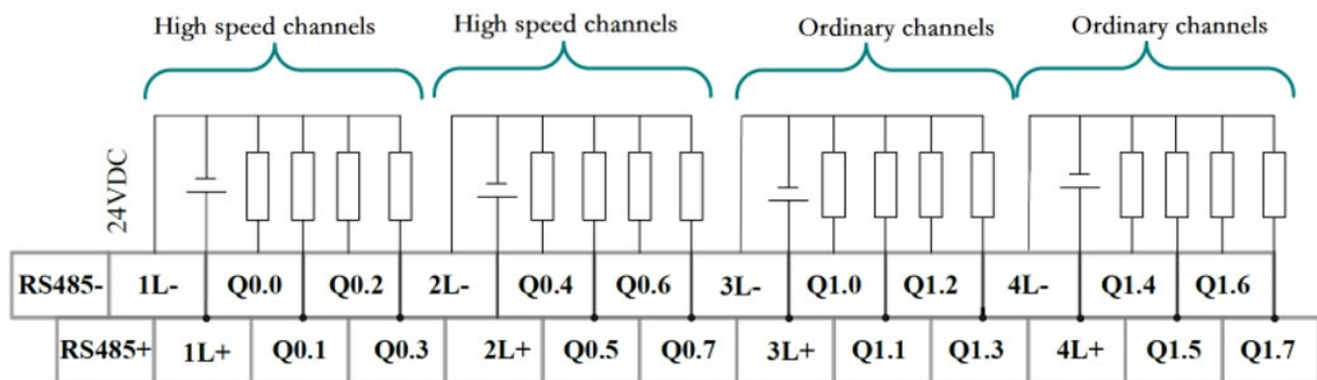
Figure 51 Lower Terminal Definition and Wiring
