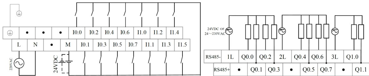
Figure 40 Upper Terminals Definition and Wring Diagram Lower Terminals Definition and Wring Diagram
