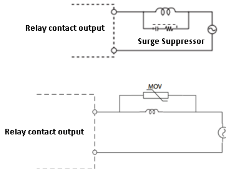
Figure 145 Typical Suppressor Circuit for Switching AC Inductive Loads
