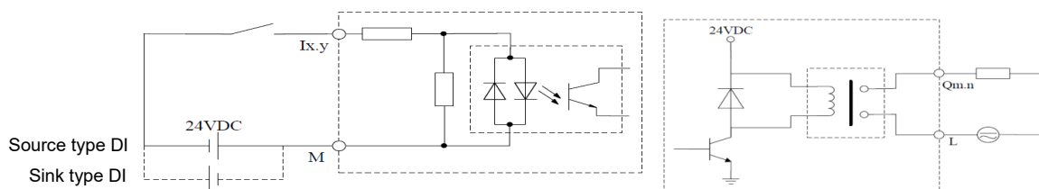
Figure 33 LE5105 input channels
