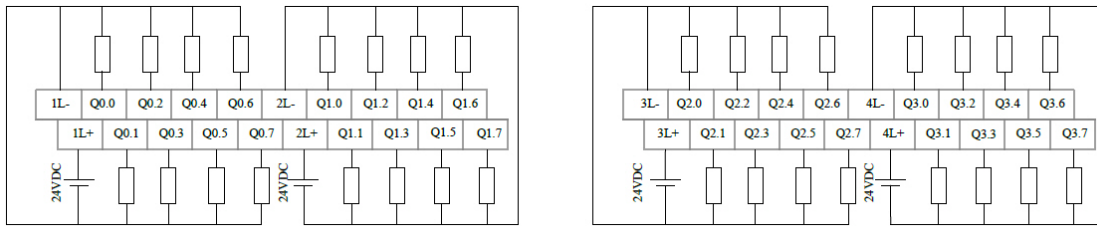
Figure 85 Upper Terminal Definition and Wiring
