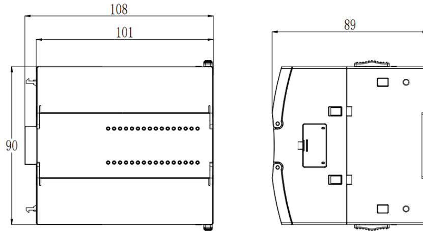
Figure 152 Outline Dimensions
