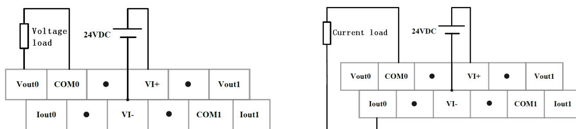
Figure 103 Upper Terminal (Voltage load) Upper Terminal (Current load)
