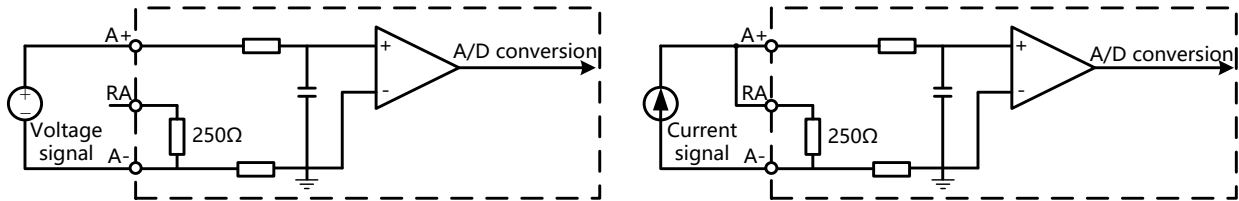
Figure 15 Analog Differential Input Channels
