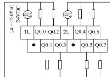
Figure 89 Upper Terminal Definition and Wiring Lower Terminal Definition and Wiring
