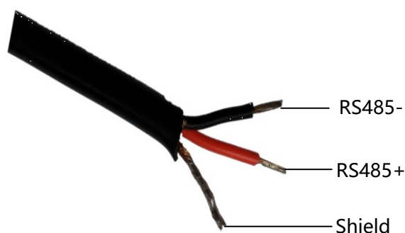
Figure 128 Wire Schematic
