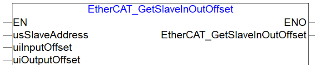
EtherCAT_GetSlaveInOutOffset Functional Block
