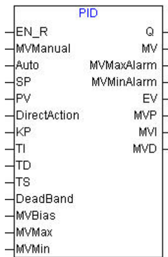
PID Functional Block
