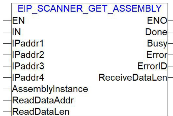
EIP_SCANNER_GET_ASSEMBLY Functional Block
