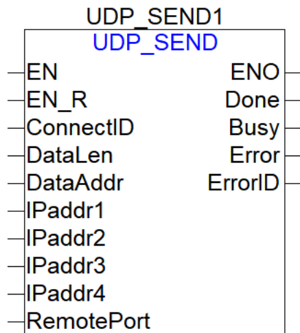
UDP_SEND Functional Block
