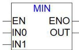
MIN Functional Block
