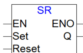
SR Functional Block
