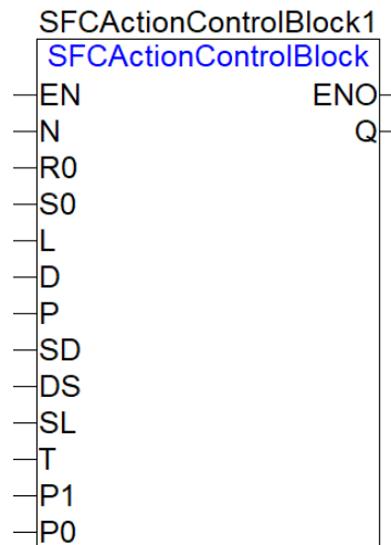
IEC Action Instruction
