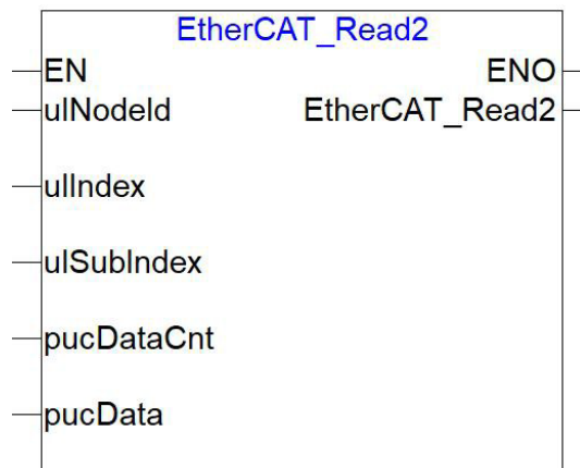
EtherCAT_Read Functional Block
