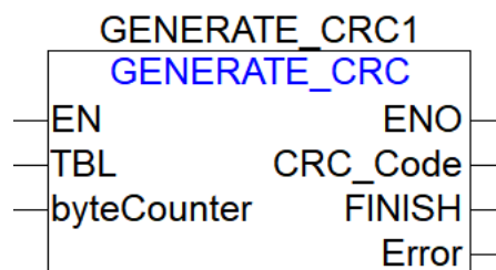
GENERATE_CRC Functional Block
