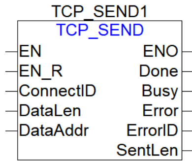
TCP_SEND Functional Block
