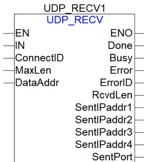
UDP_RECV Functional Block
